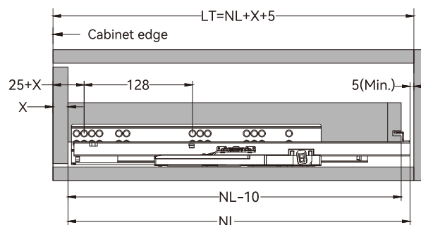
Internal drawer
