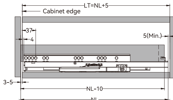
Standard drawer
